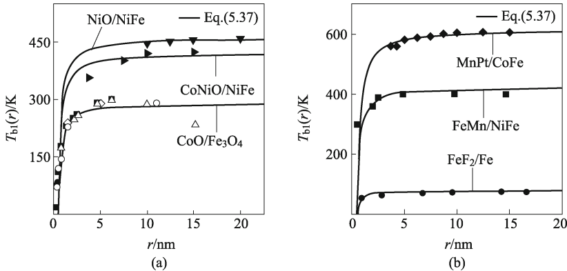
Fig. 5.15 Comparisons of T_{bl}(r) functions between Eq. (5.37) and experimental evidence: (a) \text{Fe}_3\text{O}_4/\text{CoO} (■, ◆, ●, ▲, ○, △, ◇), \text{NiO}/\text{NiFe} (▼) and \text{CoNiO}/\text{NiFe} bilayers (▶); (b) \text{FeMn}/\text{NiFe} (■), \text{MnPt}/\text{CoFe} (◆) and \text{FeF}_2/\text{Fe} bilayers systems (●). The necessary parameters are listed in Table 5.3.
