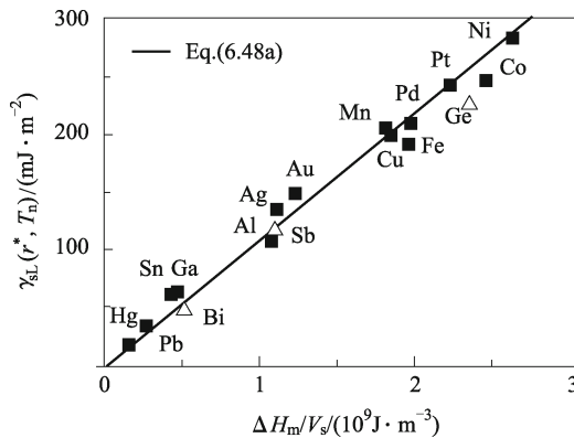
Fig. 6.14 \gamma_{\text{sL}}(r^*, T_{\text{n}}) as a function of \Delta H_{\text{m}}/V_{\text{s}} for a variety of elemental systems in terms of Eq. (6.48a) (solid line) while ■ and △ denote \gamma_{\text{sL}}(r^*, T_{\text{n}}) values of metals and semiconductors. (Reproduced from Ref. [3] with permission of Elsevier)
