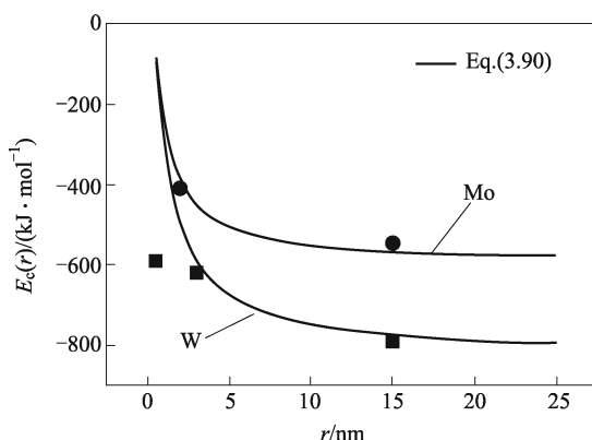
Fig. 3.12 The size dependence of E_c(r) for Mo and W nanocrystals where the solid lines denote Eq. (3.90) and the symbols \bullet [ E_c(r=2\text{nm}) = -410 \text{ kJ}\cdot\text{mol}^{-1} , E_c(r=15 \text{ nm}) = -544 \text{ kJ}\cdot\text{mol}^{-1} ] and \blacksquare [ E_c(r=0.5 \text{ nm}) = -590 \text{ kJ}\cdot\text{mol}^{-1} , E_c(r=3 \text{ nm}) = -619 \text{ kJ}\cdot\text{mol}^{-1} , E_c(r=15 \text{ nm}) = -791 \text{ kJ}\cdot\text{mol}^{-1} ] show experimental data of Mo and W nanocrystals, respectively. (Reproduced from Ref. [12] with permission of Bentham Science Publishers Ltd.)
