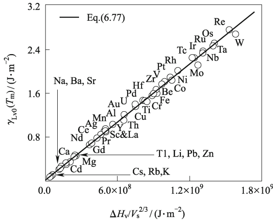
Fig. 6.19 \gamma_{Lv0}(T_m) as a function of \Delta H_v/V_s^{2/3} for liquid metals in terms of Eq. (6.77) where the solid line is linearly regressed. (Reproduced from Ref. [3] with permission of Elsevier)
