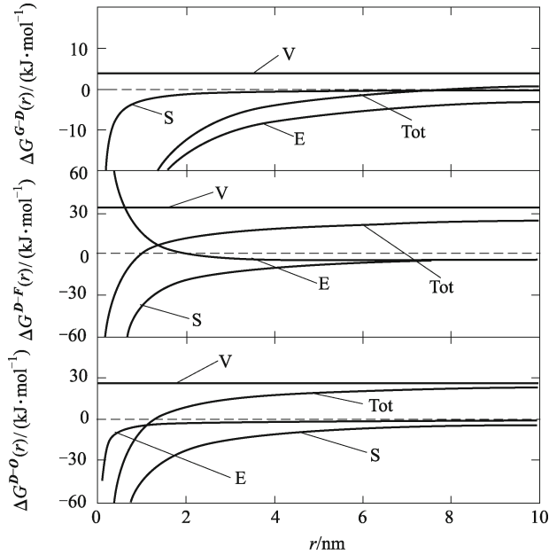
Fig. 6.28 \Delta G as a function of r where the solid lines for \Delta G^{i \rightarrow j}(T = 0, r) , \Delta G_s^{D \rightarrow j}(r) , \Delta G_e^{D \rightarrow j}(r) , and \Delta G_v^{D \rightarrow j}(T = 0) functions (simplified to Tot, S, E, and V) are determined in terms of Eqs. (6.86), (6.87), (6.90), and (6.95)–(6.98), respectively. The dotted line denotes \Delta G^{i \rightarrow j} = 0 . (Reproduced from Ref. [3] with permission of Elsevier)
