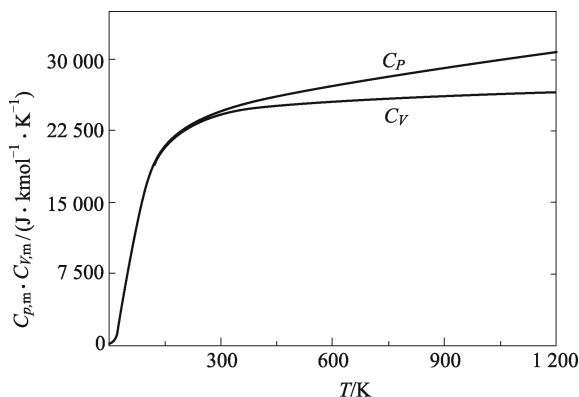
Fig. 3.2 Schematic graphs of C_{V,m} and C_{P,m} of Cu as a function of T at P = 0.1 MPa.
