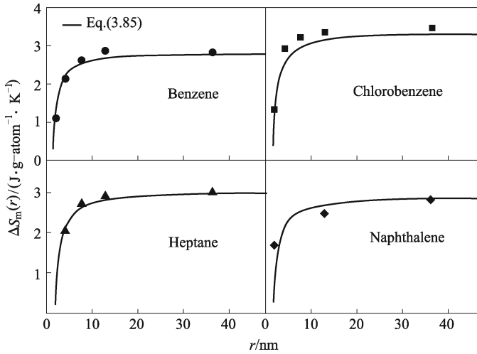
Fig. 3.9 \Delta S_m(r) functions of benzene, chlorobenzene, heptane, and naphthalene. The lines are Eq. (3.85). ●, ■, ▲, and ◆ denote the experimental results of benzene, chlorobenzene, heptane, and naphthalene, respectively. \Delta S_m(\infty) values of benzene, chlorobenzene, heptane, and naphthalene in \text{J}\cdot\text{g}\cdot\text{atom}^{-1}\cdot\text{K}^{-1} are 2.842, 3.375, 3.042, and 2.920, respectively. r_0 is taken as 2h (for the calculations of h values, see ref. [23]). The corresponding r_0 values in nm are 0.7584, 0.8036, 0.9650, and 0.9024.
