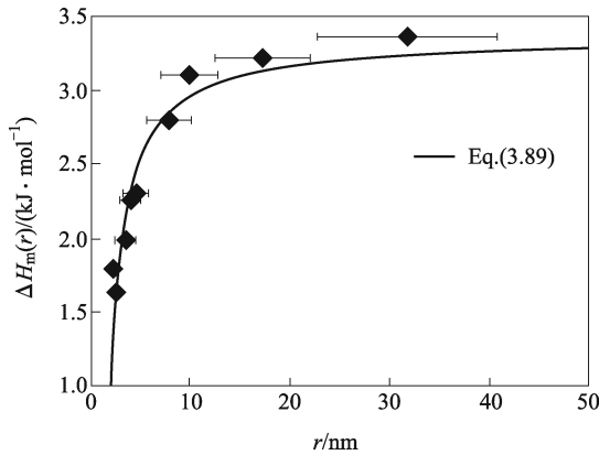
Fig. 3.11 \Delta H_m(r) functions of disk-like In nanoparticles in terms of Eqs. (3.89) shown as the solid line and the symbol \blacklozenge denotes the corresponding experimental results where \Delta H_m(\infty) = 3.36 \text{ kJ}\cdot\text{mol}^{-1} , d = 1 and other parameters are the same as the caption of Fig. 3.10. (Reproduced from Ref. [12] with permission of Bentham Science Publishers Ltd.)
