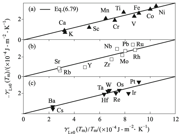
Fig. 6.20 -\gamma'_{Lv0}(T_m) as a function of \gamma_{Lv0}(T_m)/T_m for (a) the fourth ( \blacktriangle ), (b) the fifth ( \square ) and (c) the sixth ( \blacktriangledown ) periods A family metals where the solid lines are determined by Eq. (6.79). (Reproduced from Ref. [3] with permission of Elsevier)
