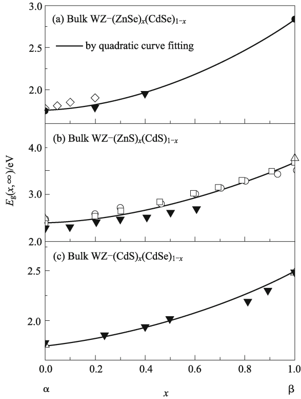
Fig. 4.13 E_g(x, \infty) functions of some bulk pseudo-binary IIB–VIB chalcogenide semiconductors of experimental (symbols) and fitting results (curves). (a) \text{WZ}-(\text{ZnSe})_x(\text{CdSe})_{1-x} , (b) \text{WZ}-(\text{ZnS})_x(\text{CdS})_{1-x} , (c) \text{WZ}-(\text{CdS})_x(\text{CdSe})_{1-x} . The mean \omega(x, \infty) values for \text{WZ}-(\text{ZnSe})_x(\text{CdSe})_{1-x} , \text{WZ}-(\text{ZnS})_x(\text{CdS})_{1-x} , and \text{WZ}-(\text{CdS})_x(\text{CdSe})_{1-x} are respectively identified as -0.92 eV, -1.01 eV and -0.50 eV by quadratic curve fitting. The curves are shown in terms of Eq. (4.27) using the mean \omega(x, \infty) values derived from quadratic curve fitting and E_g(0, \infty) and E_g(1, \infty) values listed in Table 4.4. (Reproduced from Ref. [29] with permission of Wiley-VCH)
