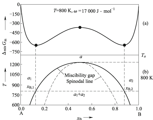
Fig. 4.8 Plots of \Delta_{\text{mix}} G_{\text{m}} versus x_{\text{B}} for a regular solution (a) and the corresponding phase diagram having the miscibility gap, showing spinodal line (b).
