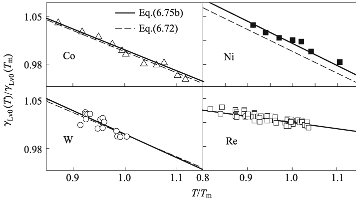
Fig. 6.22 Comparison of \gamma_{Lv0}(T)/\gamma_{Lv0}(T_m) function between the predictions of Eq. (6.75b) (solid line), Eq. (6.72) (dash line) and available experimental data for transition metals Ni (■), Co (△), Re (□) and W (○). (Reproduced from Ref. [3] with permission of Elsevier)
