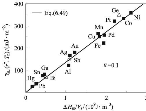
Fig. 6.15 \gamma_{\text{sL}}(r^*, T_n) as a function of \Delta H_m / V_s with \theta_c = 0.1 for elements in terms of Eq. (6.49) (solid line) where ■ and △ denote the \gamma_{\text{sL}}(r, T) values of fcc and non-fcc elements, respectively. (Reproduced from Ref. [3] with permission of Elsevier)
